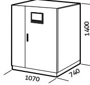
MPM/MPT 60HC÷80HC MPT 60D÷80D MPT 60DHC÷80DHC
